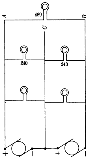
Diagram of three-wire system.
